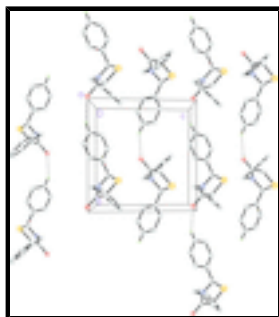
Fig. 2. The crystal packing of the title compound, viewed along the a axis.
