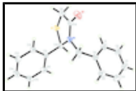
Fig. 1. An ORTEP view of the title compound, showing 30% probability displacement ellipsoids.
